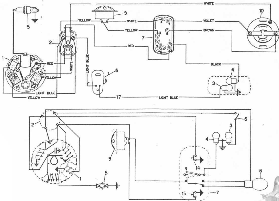
Fig. 7 - Scheme of Electric Wiring
